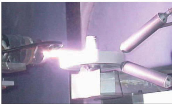
5: Plasma-Spraying
