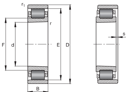
Hybrid Cylindrical Roller Bearings d 30–45 mm
