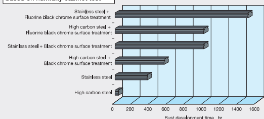
Corrosion resistance comparison based on humidity cabinet test
