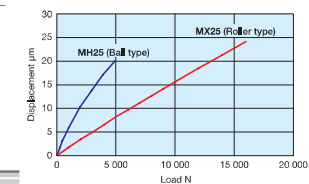
Comparison of elastic deformation
