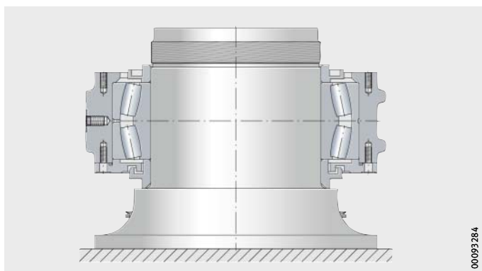
Figure 13 Mounting of the labyrinth ring for the gearbox side
